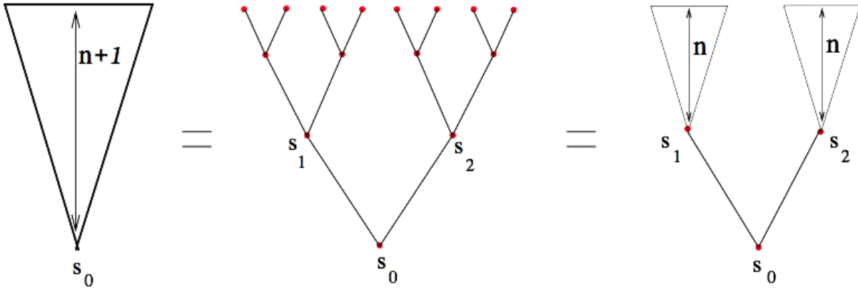
Figure 2. The recursion relation for the local magnetic field on the root of a rooted tree, here for the case K = 2 .
