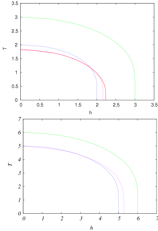
Figure 3. Top: the phase diagram of the ferromagnet in a transverse field, on a Bethe lattice with K + 1 = 3 neighbours per spin. The plot shows the critical temperature versus transverse field, separating the low- T ferromagnetic region from the high- T paramagnetic one. The full red curve is the exact result obtained by continuous-time spin trajectory population dynamics [39]. The green long dashed curve is the naive mean-field result. The blue dashed line is the result from the cavity-mean-field approximation. The dotted purple curve is the result obtained from the projected cavity mapping. Bottom: same plots with K + 1 = 6 (without the exact result), showing that the approximation going from the projected cavity mapping to the cavity-mean-field improves at larger K , as expected, and becomes rather accurate already for this moderate value of K .
