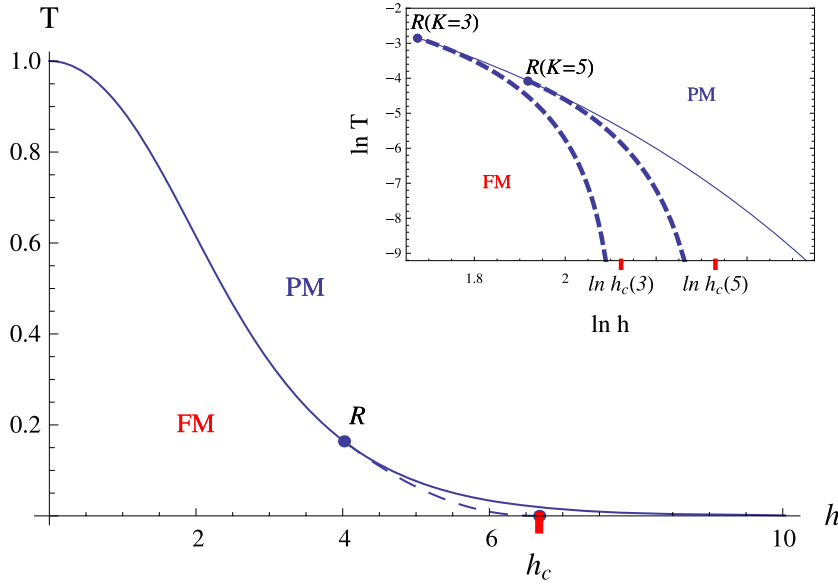
Figure 4. Phase diagram of the quantum ferromagnet in a random transverse field, as found with the RS cavity method, in the plane of the disorder strength h and the temperature T . The RS transition line (solid) is determined by the condition on the convex function: f(x = 1, T, h) = 0 , and separates the ferromagnetic (FM) state ( f(x = 1, T, h) < 0 ) from the paramagnetic (PM) state ( f(x = 1, T, h) > 0 ). The point R on the RS line corresponds to the minimum of the convex function: f'_x(x = 1, T, h) = 0 . It is the beginning of the RSB transition line, determined by the minimum of the convex function in the RSB ( x^* < 1 ) phase: f(x^*, T, h) = 0 and f'_x(x^*, T, h) = 0 . The inset shows details of the RSB lines in the cases K = 3 and 5 . The critical values of disorder h_c(K) , at which the zero-temperature quantum phase transition to the paramagnetic phase happens, for the two connectivity numbers K are h_c(K = 3) = 8.36 and h_c(K = 5) = 10.28 .
