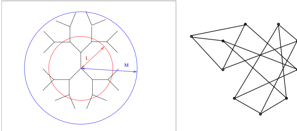
Figure 1. Left: the usual construction of the Bethe lattice. Right: a (small) random regular graph. The local structure in large random regular graph is tree-like, as in the centre of a Bethe lattice.
