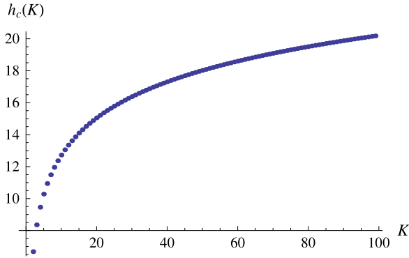
Figure 5. The critical value of disorder h_c(K) as a function of the connectivity number K .
