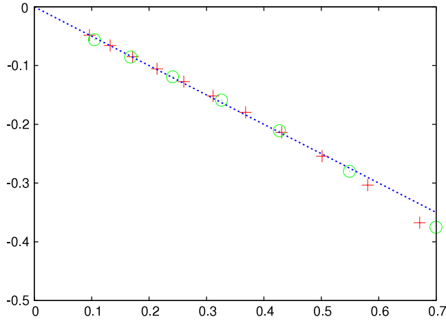
Figure 6. Phase transition in the RTFF model with K = 3 , a uniform distribution of couplings J on [0, 1] and a uniform distribution of fields \xi on [0, h] . The typical value of the local field B , measured as \exp(-\overline{\ln B}) , is plotted versus (h_c/h)^m - 1 . The crosses are obtained with the cavity-mean-field approximation and the choice h_c = 12.53 obtained from the analytic study of the DPRM problem, which predicts a linear dependence \exp(-\overline{\ln B}) = C[(h_c/h)^m - 1] . The circles are obtained with the projected cavity mapping and a fitted value h_c = 7.5 . In both cases the exponent m is the one found from the DPRM analysis, m = 0.679 . The straight line is a guide to the eye.
